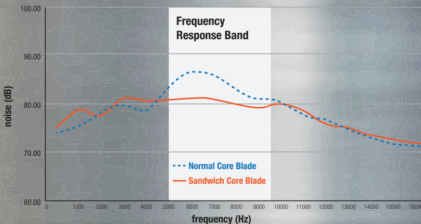
Normal Core & Silent Core Noise Comparison Test
